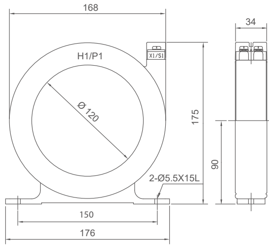
FIG.3 CG-PVB
