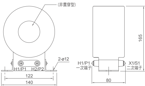
FIG.1 CG-P5 (繞線型)
